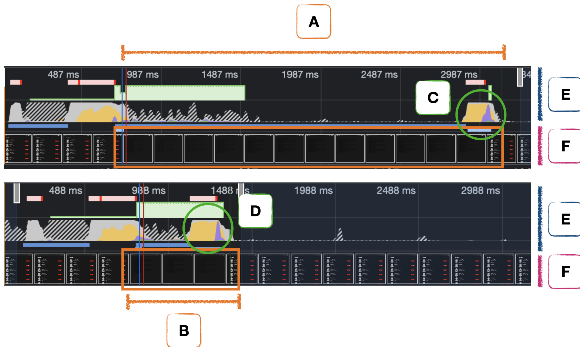
Figure 6: Two screenshots from the Chrome DevTools’ Performance Tab profiling a search turning up 100 users in youtube-clone. The profile corresponding to the original code is on top, and the refactored one is on the bottom. The two (E) labels show time series of application activity, where higher values correspond to more CPU cycles. (C) and (D) show spikes in activity when the HTTP response was received by the client before and after refactoring, resp. The two (F) labels show a series of screenshots taken of the front-end as it loads and is populated by data. (A) and (B) show the period that the screen was idle before and after refactoring, resp., and the two boxes in the timelines highlight that the screen is empty during that span.
